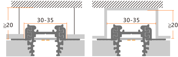
Item no.: KLM-GD4822Y/L1000 Cut hole: W30*H20mm
