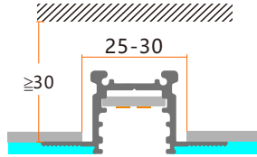
Item no.: KLM-GD4520Q/L1000 Cut hole: W25*H30mm
