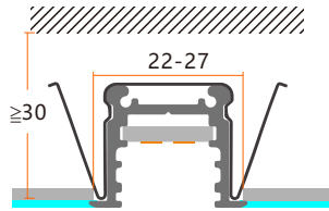
Item no.: KLM-GD2620Q/L1000 Cut hole: W22*H30mm
