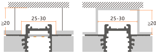
Item no.: KLM-GD4820Y/L1000 Cut hole: W25*H20mm
